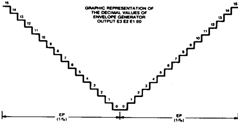
Fig. 2 DETAIL OF TWO CYCLES OF Fig. 1 (ref. waveform "1010" in Fig. 1)
