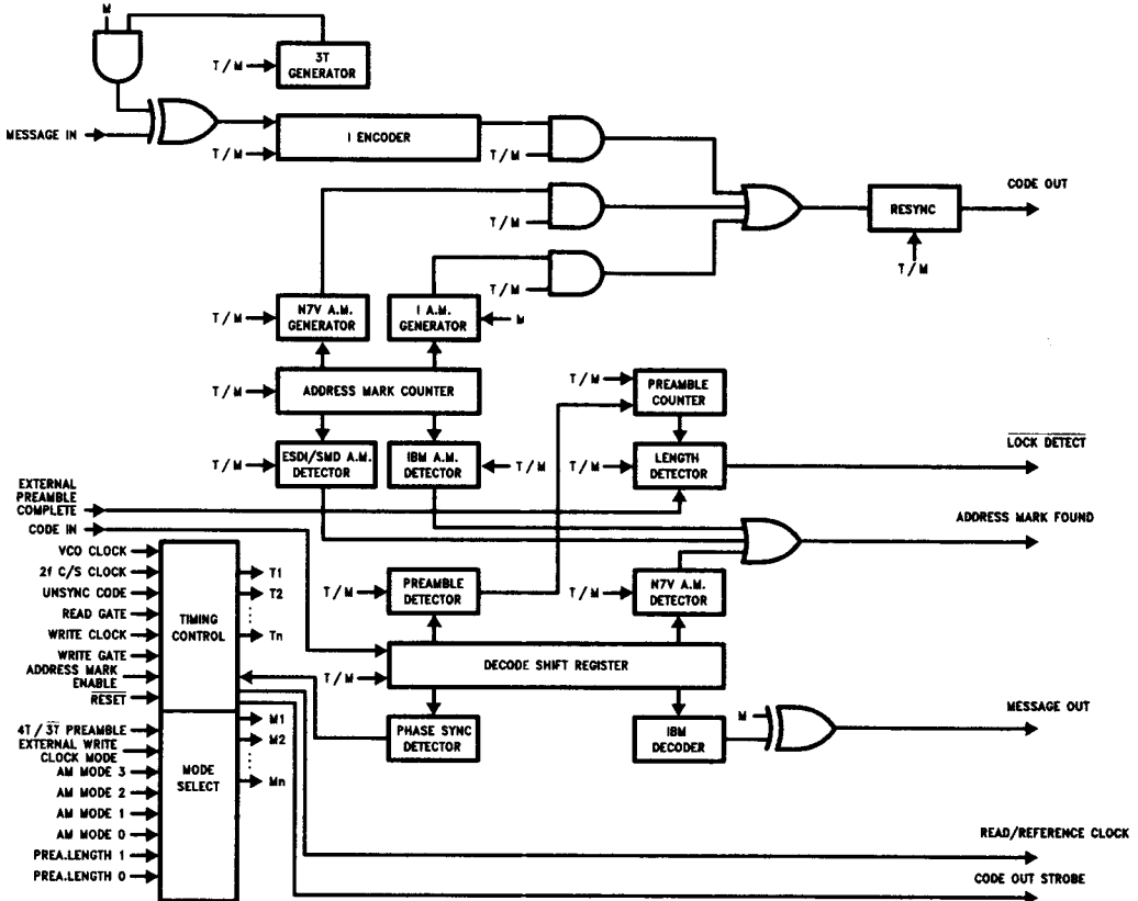
DP8463B (2, 7) Endec Block Diagram
