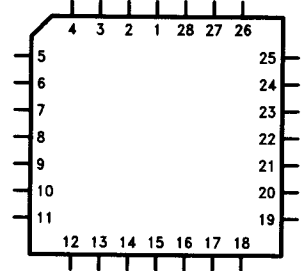
Plastic Chip Carrier (Signal Assignments to the Pin Numbers are identical to DIP)
