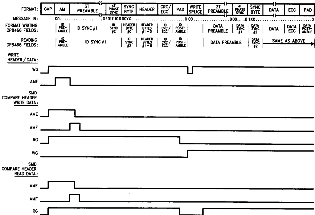
FIGURE 1-3i. ESDI, SMD, or IBM AM, 3T Preamble
