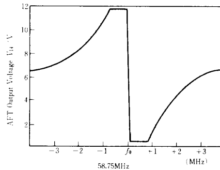
AFT OUTPUT VOLTAGE vs. FREQUENCY
