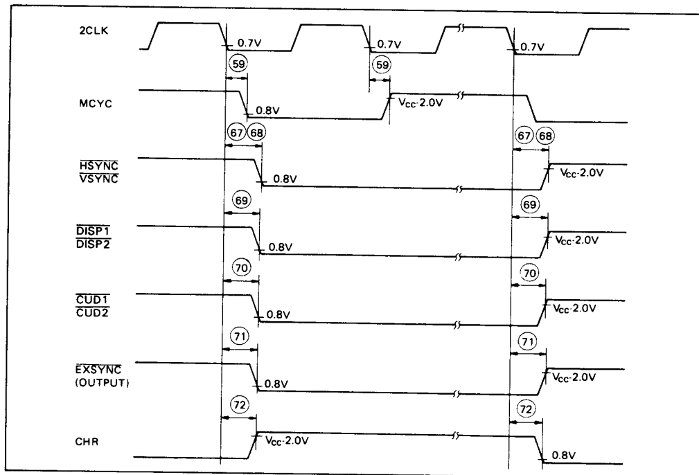
Figure 29. Display Control Signal Output Timing
