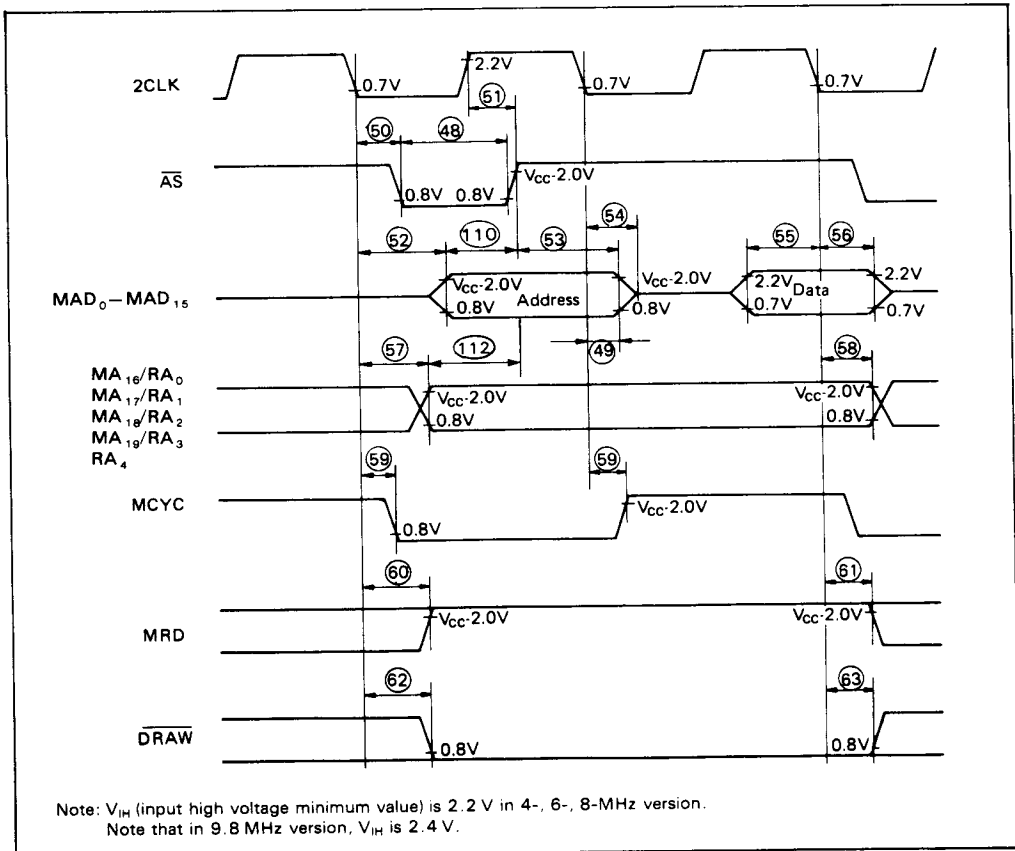
Figure 26. Frame Memory Read Cycle Timing (ACRTC - Frame Memory)
