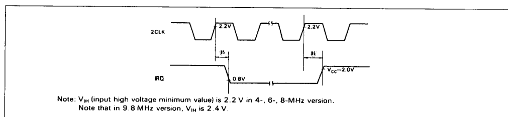
Figure 34. IRQ Output Timing
