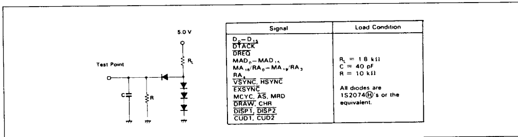
Figure 36. Test Load Circuit A
