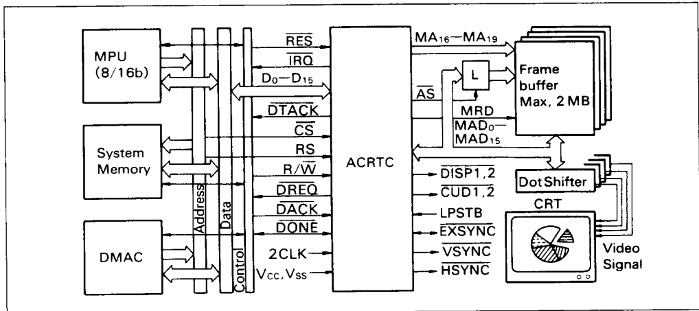
Figure 2 System Configuration
