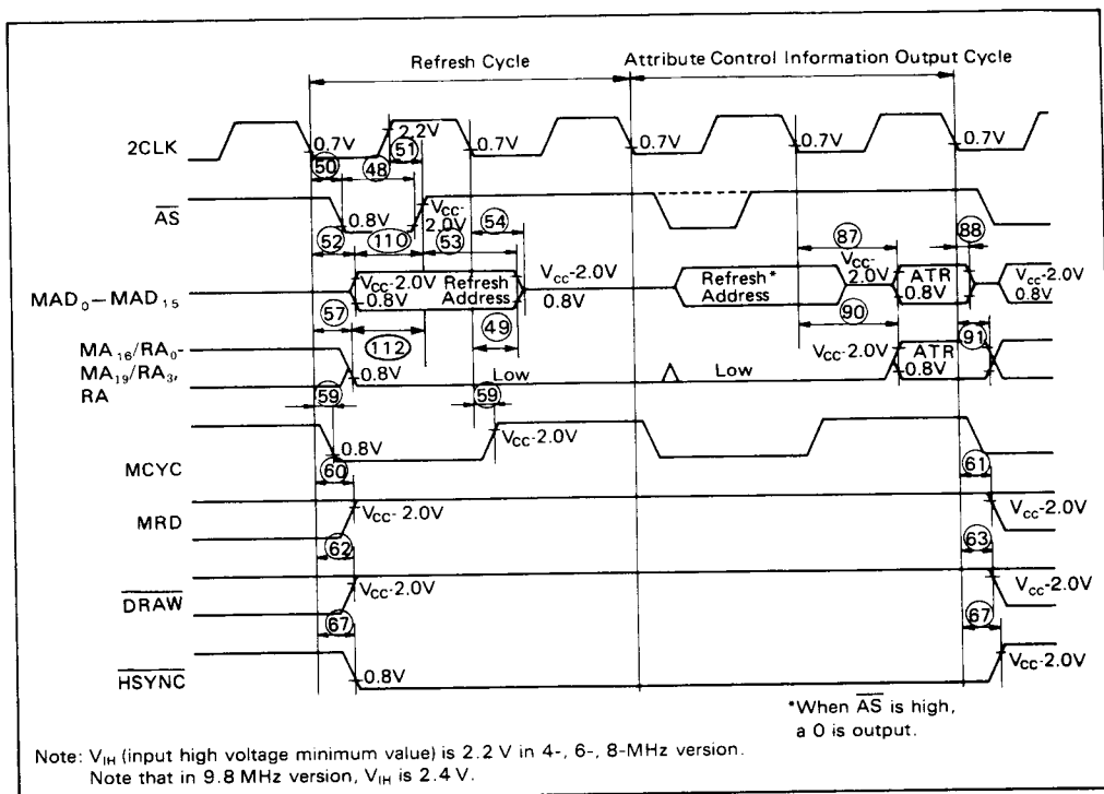
Figure 28. Frame Memory Refresh/Video Attributes Output Cycle Timing
