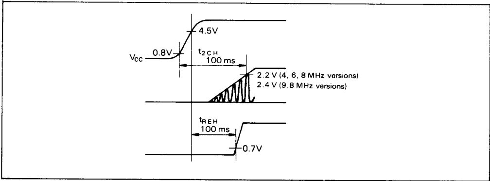
Figure 10. Power-On Sequence
