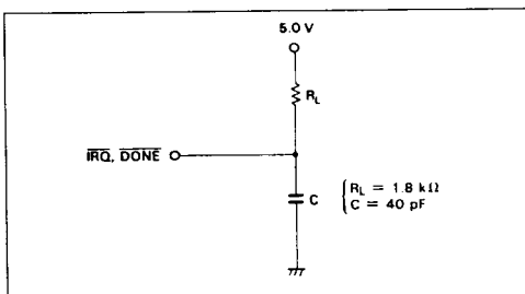
Figure 37. Test Load Circuit B
