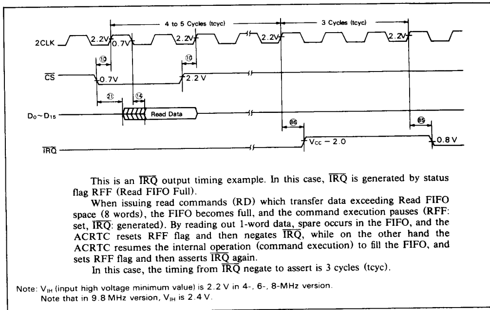
Figure 35. \overline{\text{IRQ}} Output Timing (Example: Read FIFO Full Interrupt Enable)
