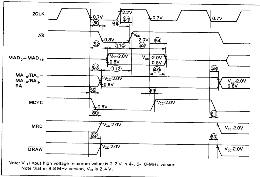
Figure 25. Display Cycle Timing
