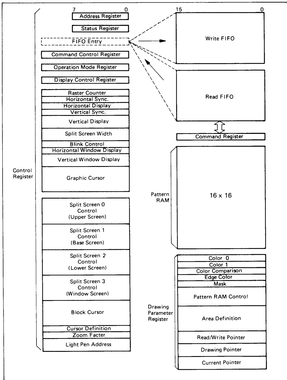
Figure 4. Programming Model
