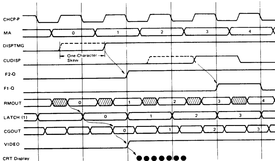
Figure 25 Time Chart of Display Control Unit (2)
