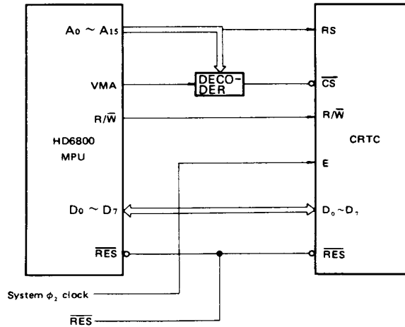
Figure 17 Interface to MPU
