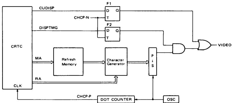
Figure 21 Display Control Unit (1)
