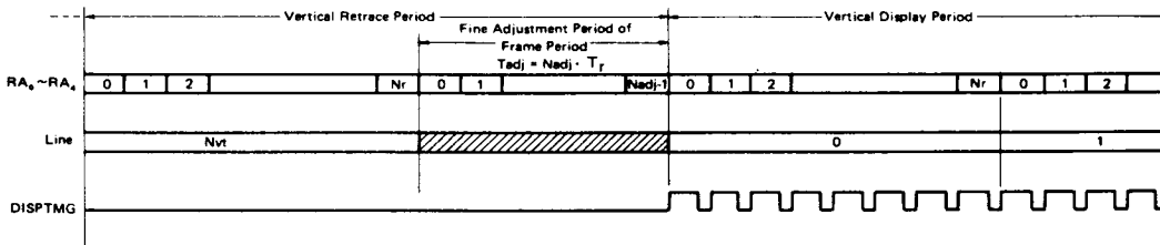
Figure 12 Fine Adjustment Period of Frame in Vertical Display (Expansion of Fig. 10— Ⓑ )
