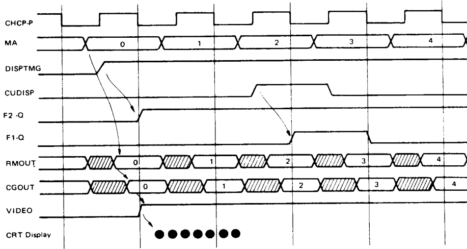
Figure 24 Time Chart of Display Control Unit (1)
