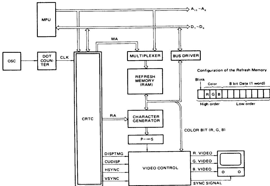
Figure 33 Color Character Display
