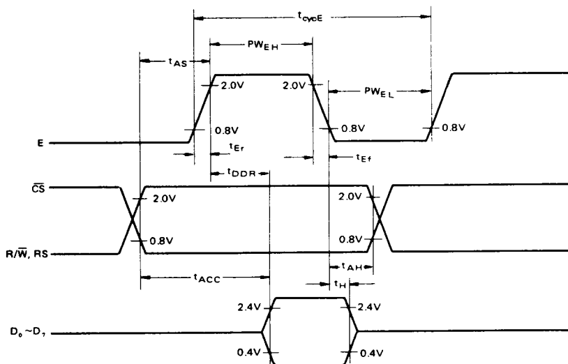
Figure 3 Read Sequence
