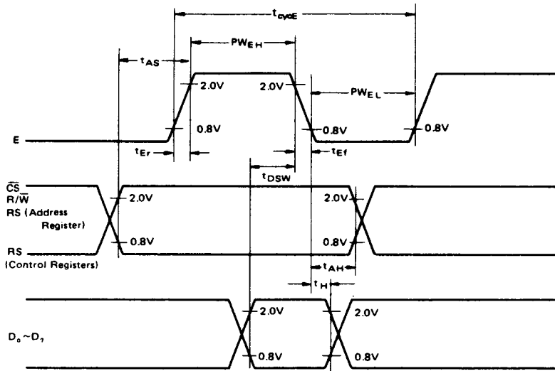
Figure 4 Write Sequence
