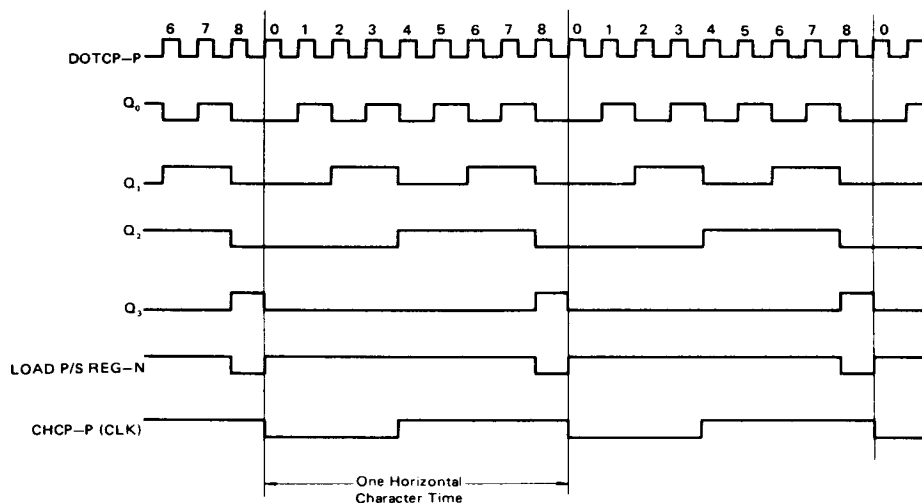
Figure 19 Time Chart of Dot Counter
