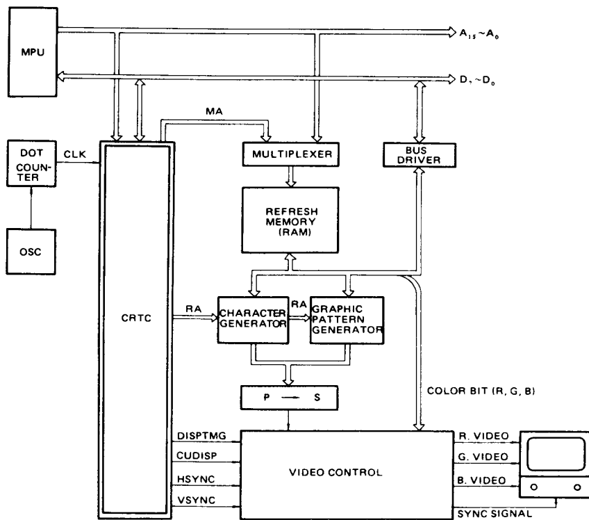
Figure 34 Color Limited Graphic Display
