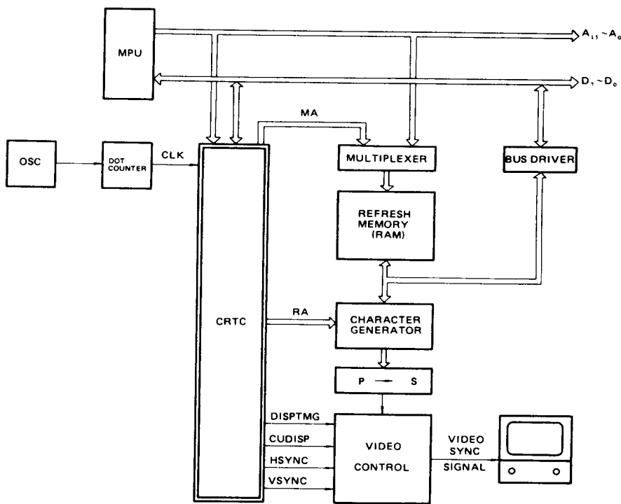
Figure 32 Monochrome Character Display
