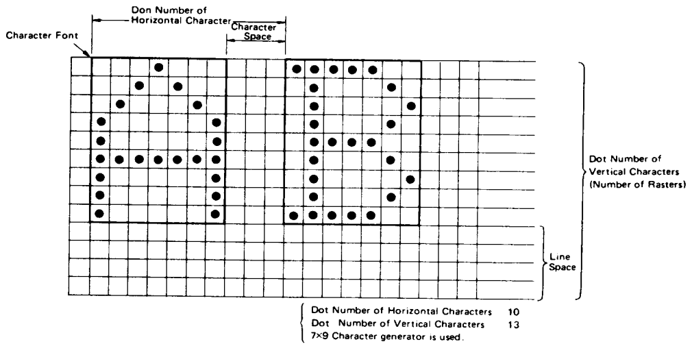
Figure 29 Dot Number of Horizontal and Vertical Characters
