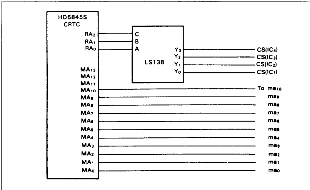
Figure 38-A Refresh Memory Address Method for Full Graphic Display
