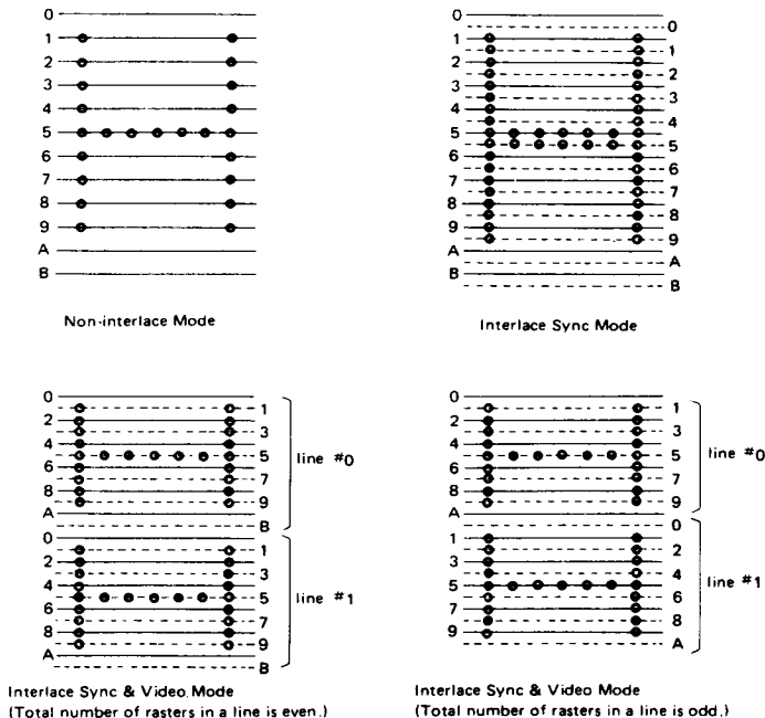
Figure 8 Example of Raster Scan Display
