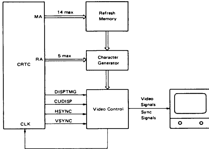
Figure 20 Interface to Display Control Unit
