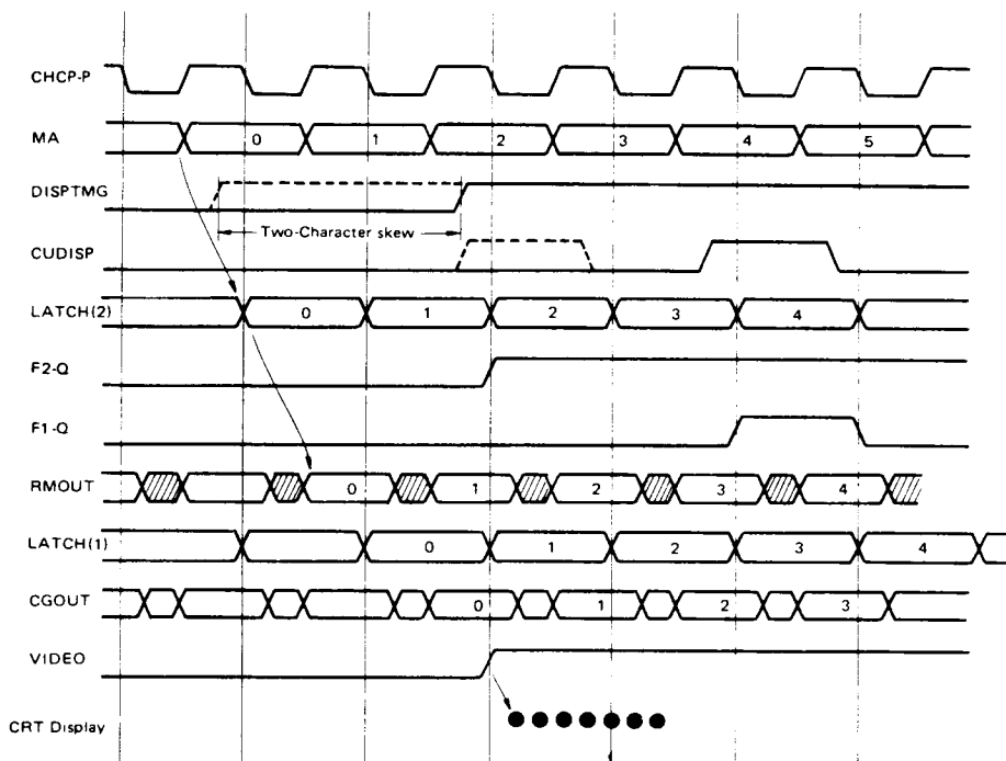
Figure 26 Time Chart of Display Unit (3)
