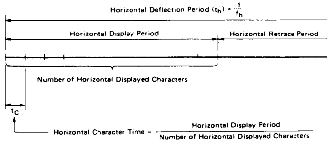
Figure 31 Number of Horizontal Displayed Characters
