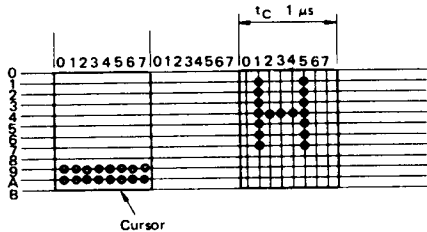
Figure 40 Non-interlace Display (Example)
