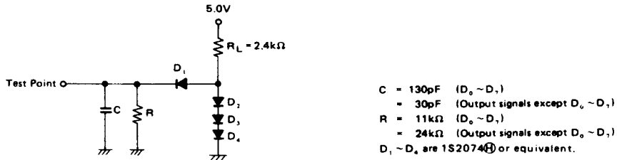
Figure 5 Test Loads
