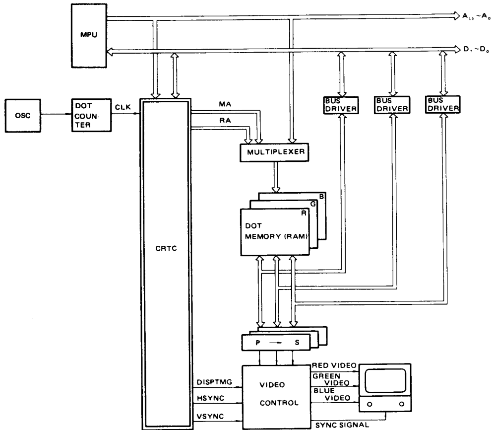
Figure 38 Color Full Graphic Display
