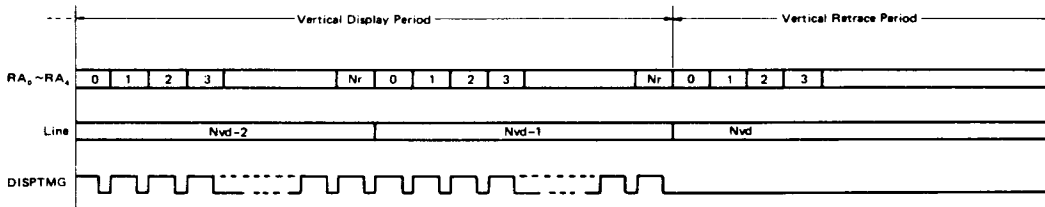
Figure 11 Switching from Vertical Display Period over to Vertical Retrace Period (Expansion of Fig. 10— Ⓐ )
