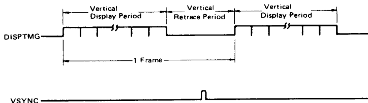
Figure 28 Time Chart of VSYNC
