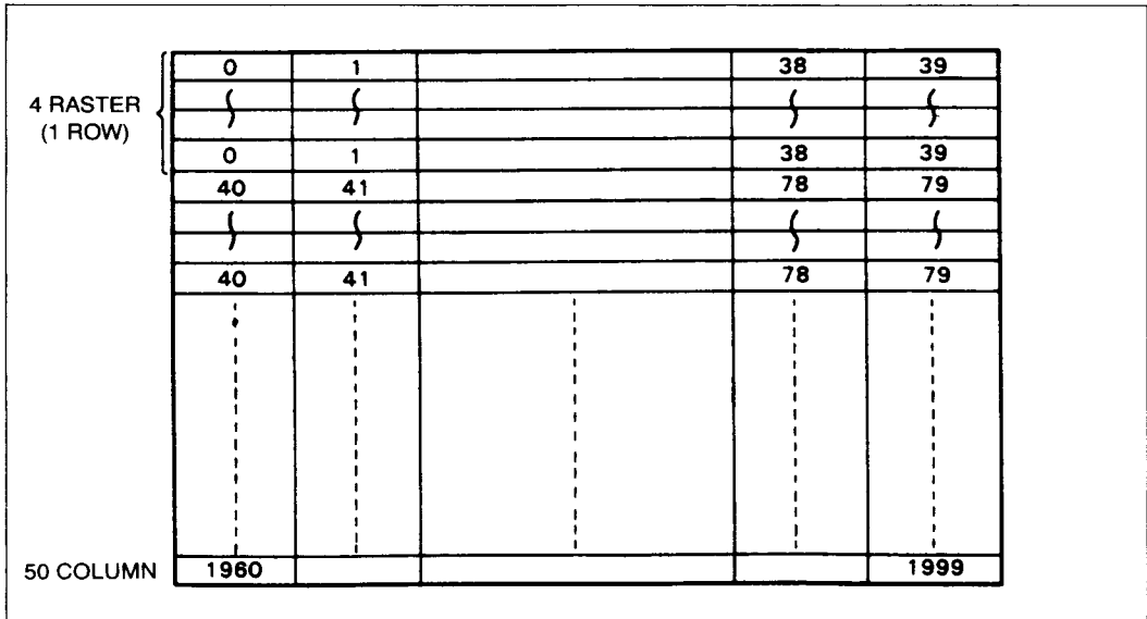
Figure 38-B Memory Address and Dot Display Position on the Screen for Full Graphic Display
