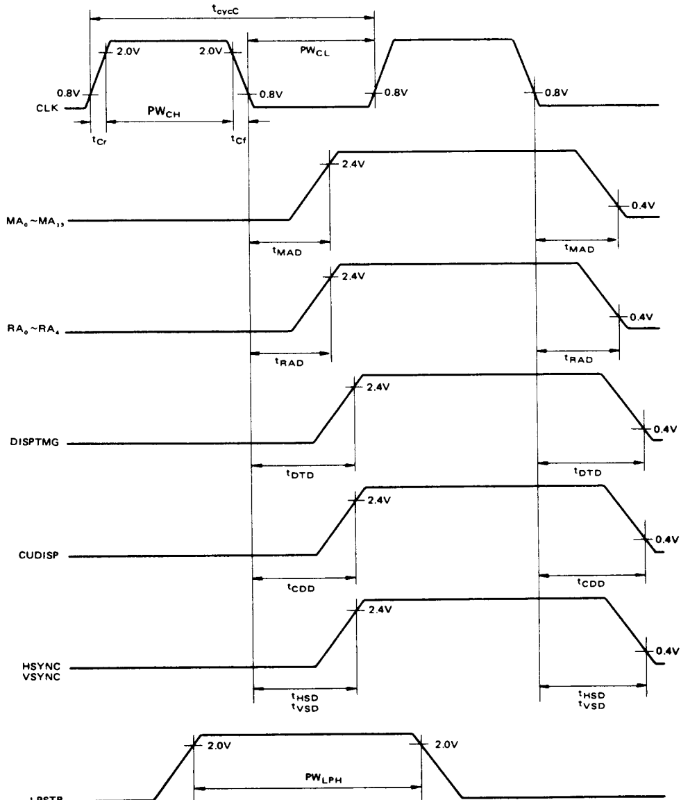
Figure 1 Time Chart of the CRTC
