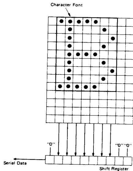
Figure 30 How to Make Character Space
