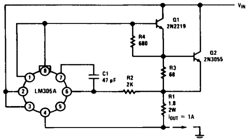
Current Regulator
