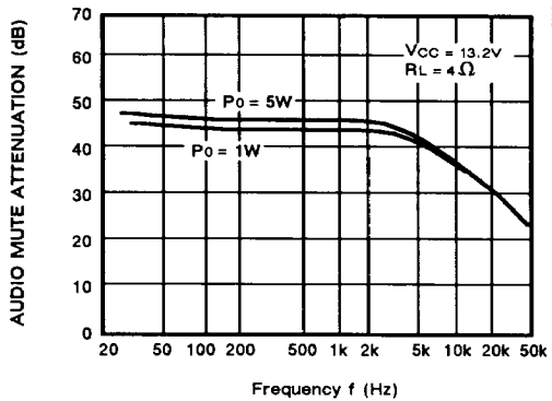
Fig. 9 - AUDIO MUTE ATTENUATION vs. FREQUENCY
