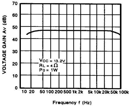
Fig. 6 - VOLTAGE GAIN vs. FREQUENCY
