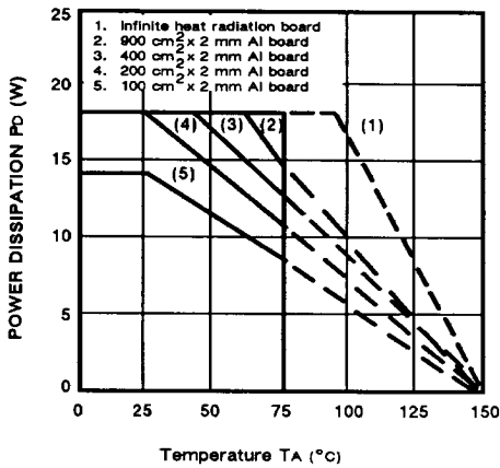
Fig. 8 - POWER DISSIPATION vs. TEMPERATURE
