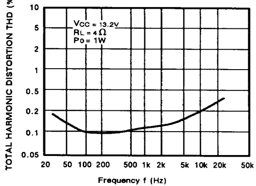
Fig. 7 - TOTAL HARMONIC DISTORTION vs. FREQUENCY
