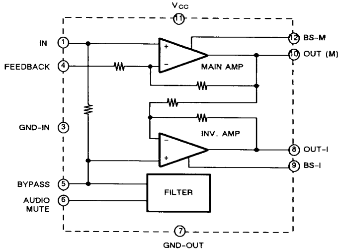
Fig. 1 - MB3731 BLOCK DIAGRAM
