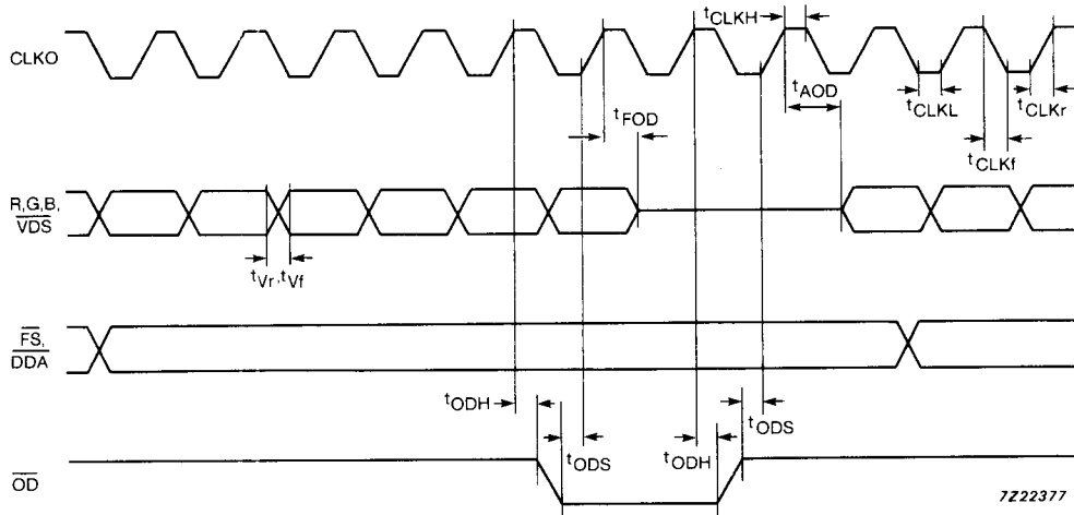
Fig. 6 Video timing.
