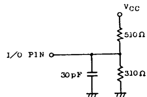
Fig.1 OUTPUT LOAD
