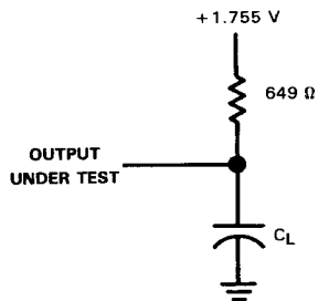
FIGURE 1 - OUTPUT LOAD
