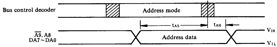
Fig. 7 Address timing
