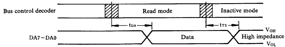
Fig. 9 Read mode
