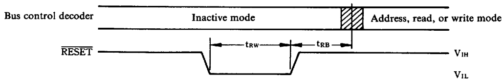
Fig. 6 Reset timing
