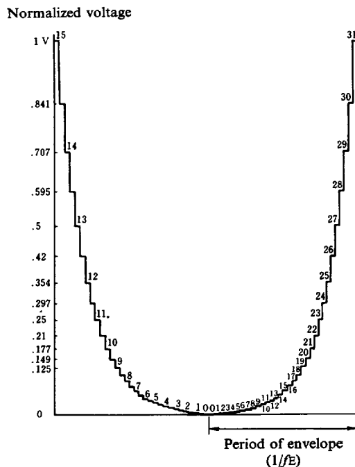
Fig. 1 Output level of DA convertor
