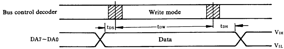
Fig. 8 Write mode
