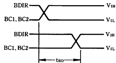
Fig. 5 Bus control timing
