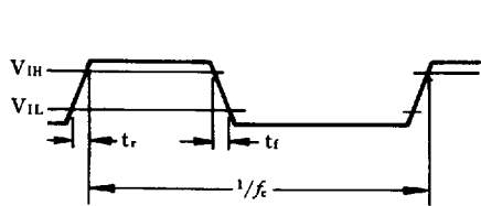
Fig. 4 Clock timing
