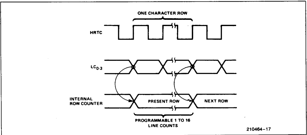
Figure 17. Row Timing
