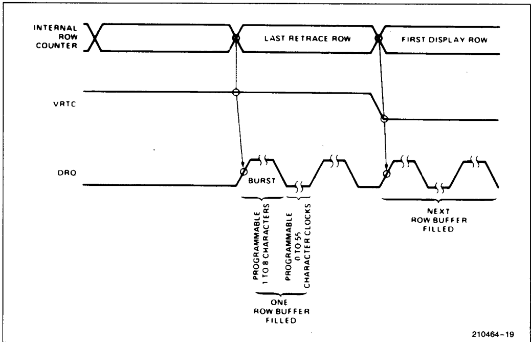
Figure 19. DMA Timing
