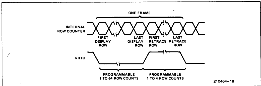
Figure 18. Frame Timing
