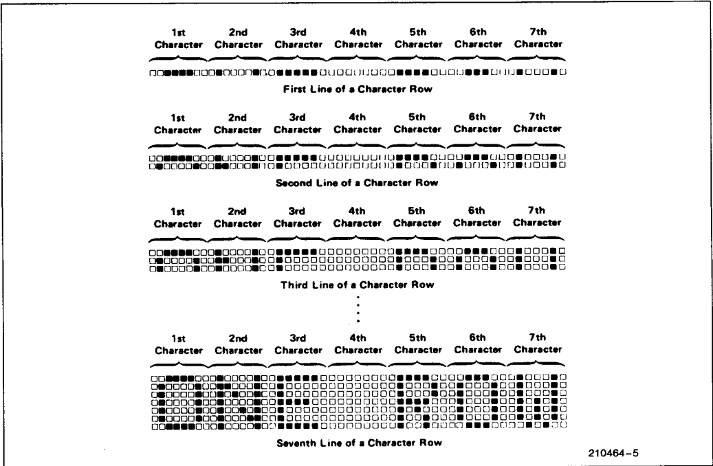
Figure 5. Display of a Character Row
