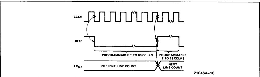
Figure 16. Line Timing
