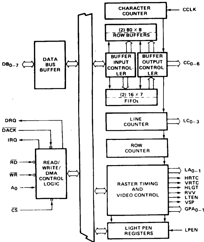
Figure 1. Block Diagram
