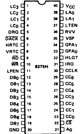
Figure 2. Pin Configuration
