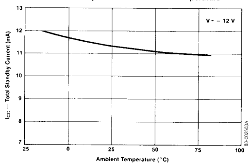
Total Standby Current vs. Ambient Temperature
