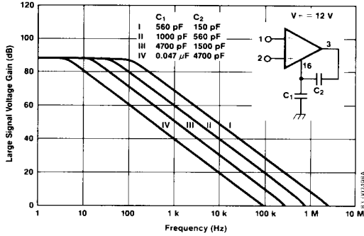
Error Amplifier I, A V1 vs. Frequency
