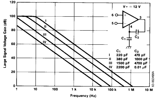
Error Amplifier II, A V2 vs. Frequency
