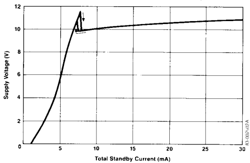
Total Standby Current vs. Supply Voltage
