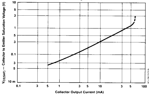
Correct Saturation Voltage vs. Collector Current
